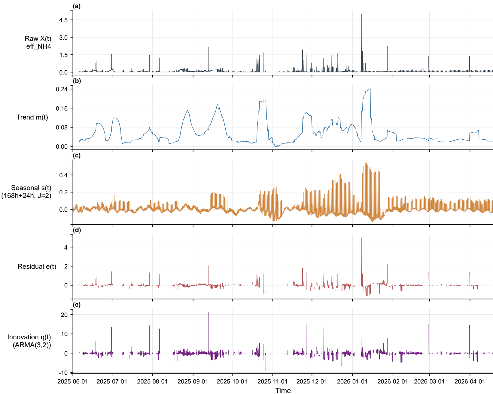
Multi-scale decomposition — eff_NH4 (effluent, hour) [2025-06-01~2026-04-19]
